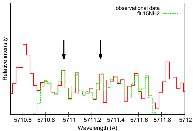
Fig. 5. ^{15}NH_2 emission lines that were detected with our observational data at 5710.959 and 5711.275 Å ((0,10,0)-(0,0,0) band)). The intensities have been averaged on 0.03 Å spectral bins, and we fitted the lines ad hoc with the ^{15}NH_2 lines located at the above-mentioned wavelengths.
