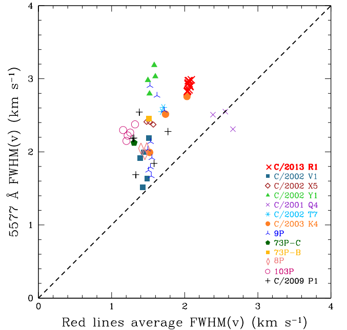
Fig. 3. 5577.339 \text{\AA} FWHM(v) against the red line average FWHM(v). Results for 12 other comets obtained from UVES spectrograph and analyzed by Decock et al. (2013) are also plotted for comparison.
