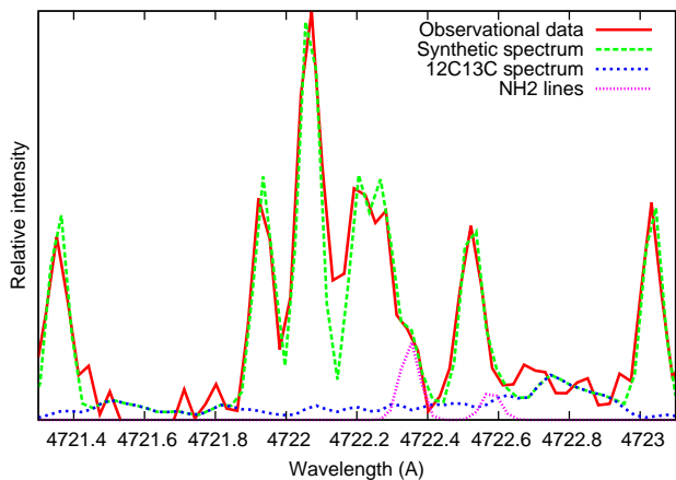
Fig. 4. C_2 and ^{12}C^{13}C emission lines corresponding to the (2,1) bandhead. Some NH_2 emission lines also appear in this region. They have been fitted with ad hoc intensities. The ^{12}C^{13}C fit corresponds to a ^{12}C/^{13}C ratio of 80. To improve the signal-to-noise ratio, the intensities have been averaged on 0.03 Å spectral bins. The (2,1) ^{12}C^{13}C bandhead appears clearly at 4722.8 Å.
