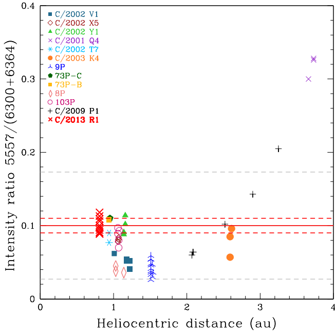
Fig. 2. G/R intensity ratio as a function of the heliocentric distance (au). Results for 12 other comets obtained from the UVES spectrograph and analyzed by Decock et al. (2013) are also plotted for comparison. The solid line represents the average value for the R1 Lovejoy spectra, and the corresponding standard deviation ( \sigma ) range is denoted with horizontal dashed lines.
