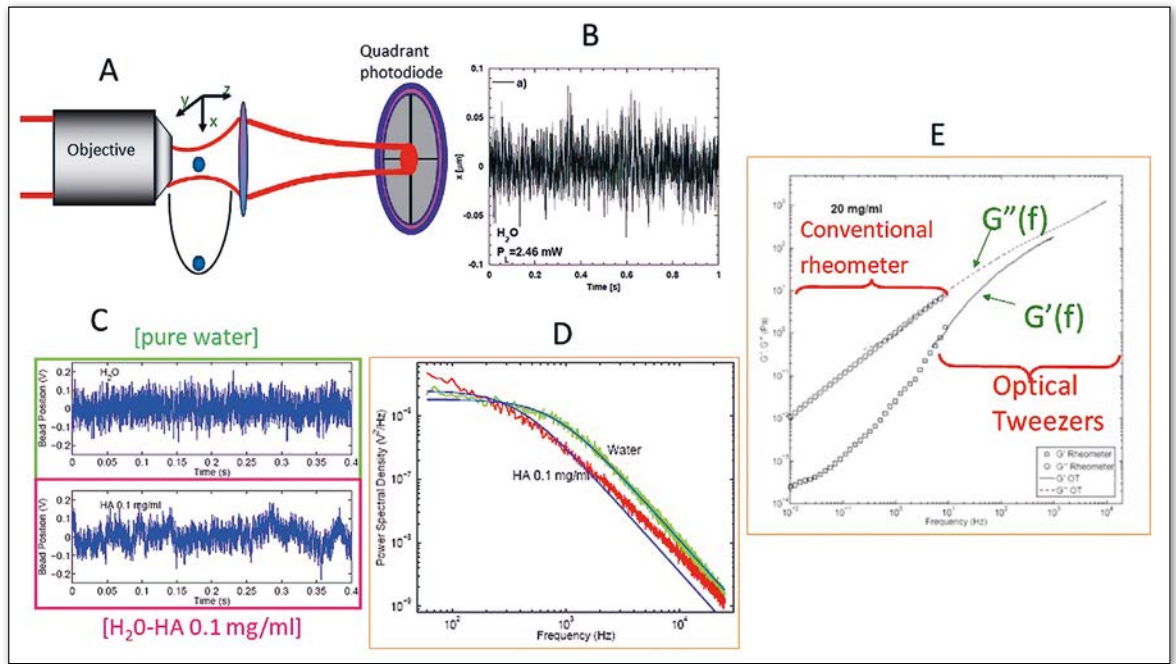
► FIG. 1: A micrometric bead is confined in the harmonic potential well of the trap (A) and its stochastic trajectory is acquired by a quadrant photodiode with accuracy of few nm (B). The stochastic traces are altered from the passage from a Newtonian fluid to a complex one, as shown in (C) and (D). Losses and elastic moduli versus the frequency as determined with conventional rheology and OT-based microrheology (E).
