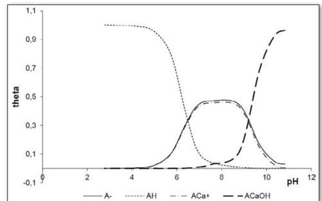
▲ Coverage of the lipid bilayer membrane surface with ions, as a function of pH.
