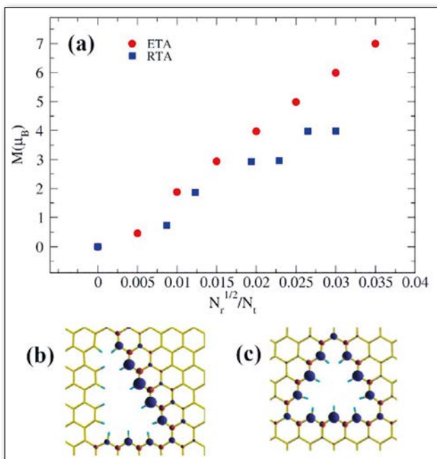
▲ Total magnetic moments of triangular holes in graphene.
