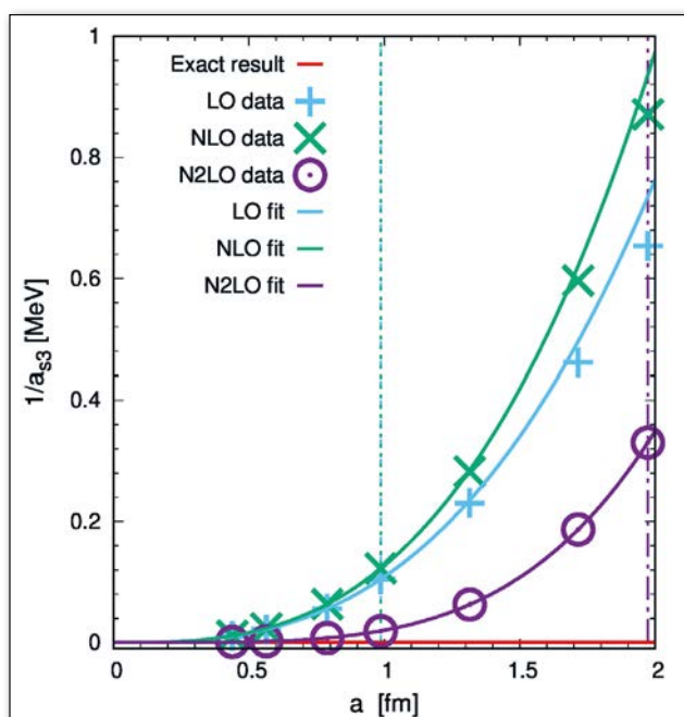
▲ The dimer-boson inverse scattering length 1/a_{s3} versus lattice spacing at LO, NLO, and N2LO. The vertical lines give the upper limits of the fit range.
