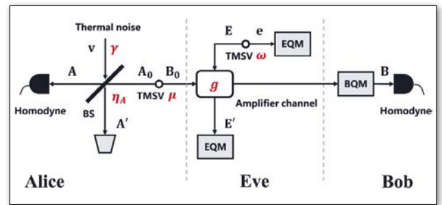
▲ Schema of the encryption channel.
